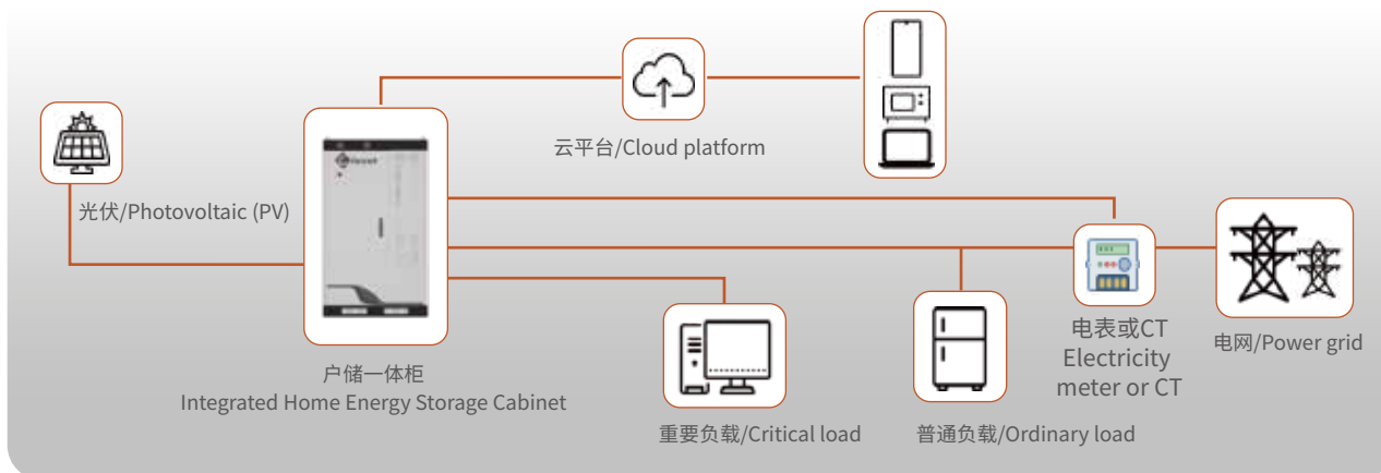
System Diagram
